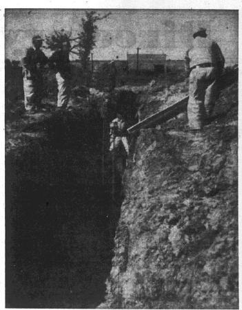
By Press-Record Staff Photographer FOOTINGS for foundation and walls at RC Cola plant being constructed on Route 67 are poured as workmen take full advantage of warmer weather. Contractor's superintendent said the project is "right on schedule." Brick work on plant offices is to begin.
